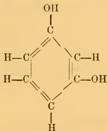
Resorcin or resorcinol.
